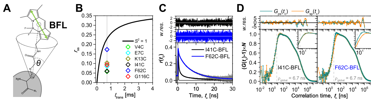
Figure 6. Fluorescence anisotropy decay and polarization-resolved FCS studies of cysteine variants of GABARAP labeled with BFL. (A) BODIPY FL (structure shown with the transition dipole moment marked by a green arrow) coupled to the side chain of cysteine. The diffusion cone is indicated with the angle \theta that is related to order parameter S^2 . (B) Relation between translational ( x -axis) and rotational ( y -axis) diffusion parameters probed with fluorescence assuming a diffusing rigid sphere, rigid attachment of the fluorophore S^2 = 1 , and the following parameters: fluorescence lifetime \tau_e = 5.35 ns, focal volume radius \omega_0 = 0.5 \mu\text{m} , and fundamental anisotropy r_0 = 0.37 (gray line, eq 37). The condition of S^2 = 1 is not achieved, and hence, the deviations of steady-state anisotropy r_{ss} from the ideal line (black) occur for all measured GABARAP variants. Note that the deviations depend on the rigidity of the fluorophore attachment ( S^2 ) (Table 1). (C) Time-resolved anisotropy r(t_c) of the variants I41C-BFL and F62C-BFL. The variant F62C is characterized by a slower anisotropy decay and larger amplitude of the global rotational diffusion term than I41C (Table S2B). As parameters were retrieved by global fitting to sum and difference curves (eq 39), the time-resolved anisotropy and weighted residuals are displayed for visualization purpose only. Analysis of \rho_{\text{global}} enables overcoming limits of the steady-state anisotropy regarding the flexibility of fluorophore attachment. (D) Cross-correlation curves G(t_c) from pFCS were fit by a rotation model ( \rho_{\text{global}} is marked by the dashed gray line). Note the difference in contrast between G_{sp}(t_c) and G_{ps}(t_c) of variants F62C-BFL and I41C-BFL (see insets for magnification) caused by the significantly higher internal mobility of the dye in the case of I41C-BFL. Top panels in (C) and (D) show the weighted residuals of the fit.
