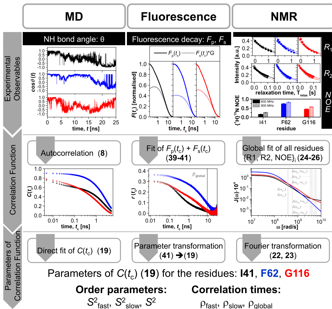
Figure 2. Workflow of the integrated analysis. Our integrated approach combines MD simulations, spectroscopic techniques based on fluorescence anisotropy and fluorescence correlation, and NMR spectroscopy. The used equations are printed in bold. The left and middle columns show for MD simulations and fluorescence spectroscopy the raw data that are monitored using these two techniques, respectively. As illustrative examples we show data for residues I41 (high flexibility, black), F62 (low flexibility, blue), and G116 (high flexibility, red), which are also discussed in detail in this paper. The raw data are processed to obtain the autocorrelation function, C(t_c) for the decay of the N–H bond vector orientation as measured by the cosine of the angle \theta(t_c) , and the fluorescence anisotropy, r(t_c) , respectively (middle row). In the case of NMR spectroscopy, the raw data are given by the spectral densities measured at two different external magnetic fields with Larmor frequencies of 600 and 900 MHz, as indicated by the gray vertical lines in the top panel of the right column. From these, the spectral densities J(\omega) are back-calculated via an iterative fitting procedure determining R_1 , R_2 , and heteronuclear NOEs (right top panel). From J(\omega) , r(t_c) , and C(t_c) the order parameters and time scales for internal and global motion can then be determined via fitting of the corresponding equations.
